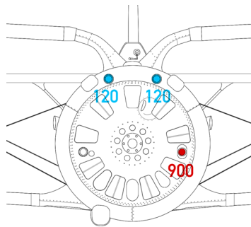
Baku #1 modification 2 x UBS 1 x ShKAS Proposal
